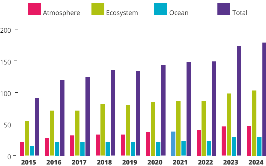
Figure 4. Number of ICOS stations in 2015–2024. The total number of stations was 179 in 2024.
