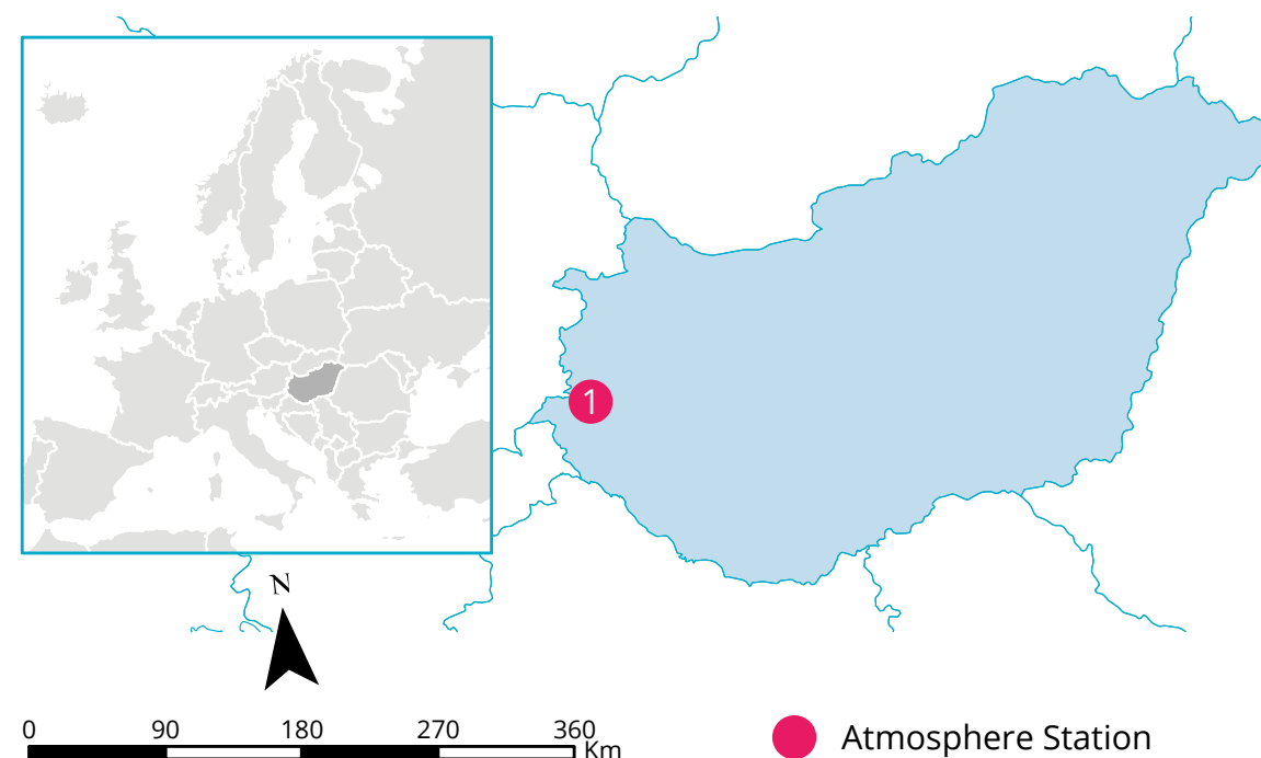
Figure 21: The ICOS Hungary station network. The numbers in the map correspond to the numbers in Table 18.
